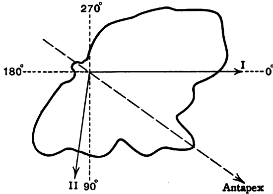
X. Region XVI. ; centre R.A. 20^{\text{h}} 24^{\text{m}} , Dec. +17^{\circ} .
